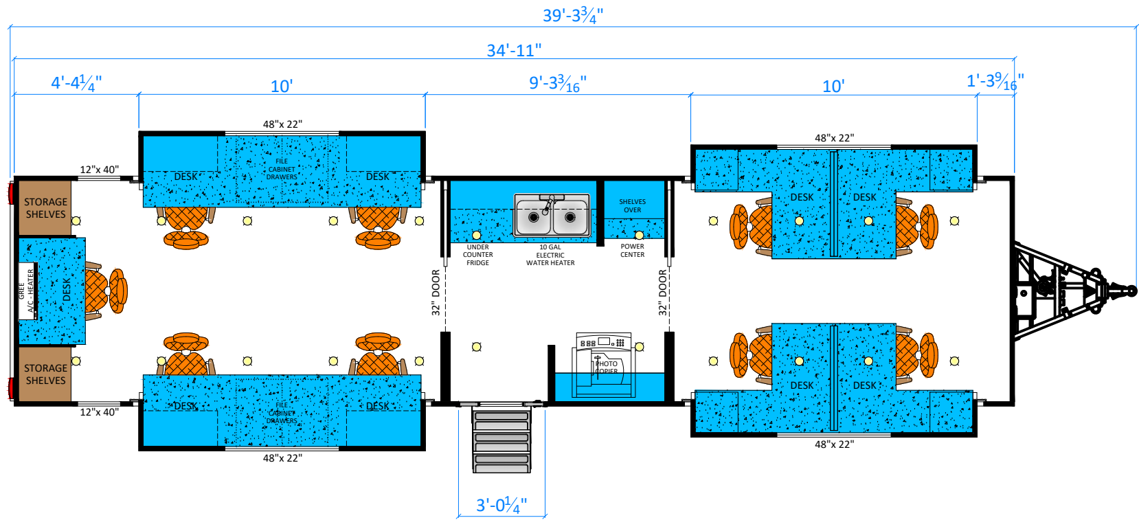
THEATRICAL TRAILERS (TYPE 3 VCA) DIAMOND PRODUCTION OFFICE TRAILER 343 SQ.FT.
