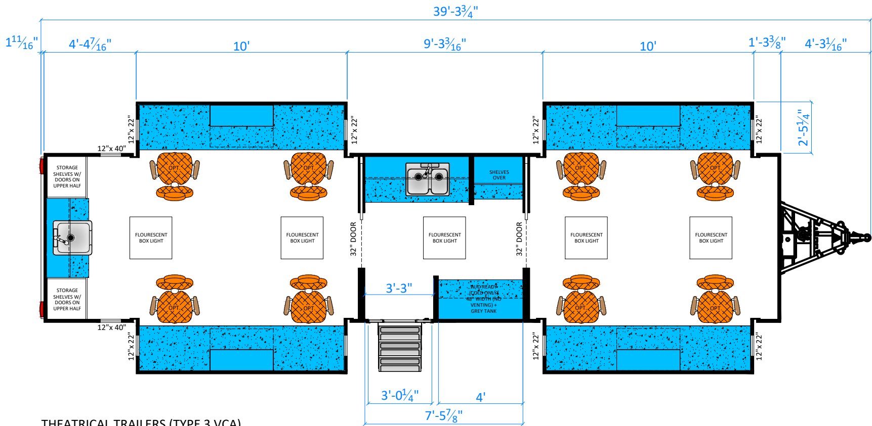
THEATRICAL TRAILERS (TYPE 3 VCA) DIAMOND MAKEUP TRAILER (8) 378 SQ.FT.
