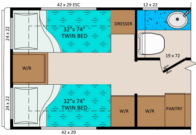
CITATION REWARD (31) 205 SQ.FT TRAVEL TRAILER
