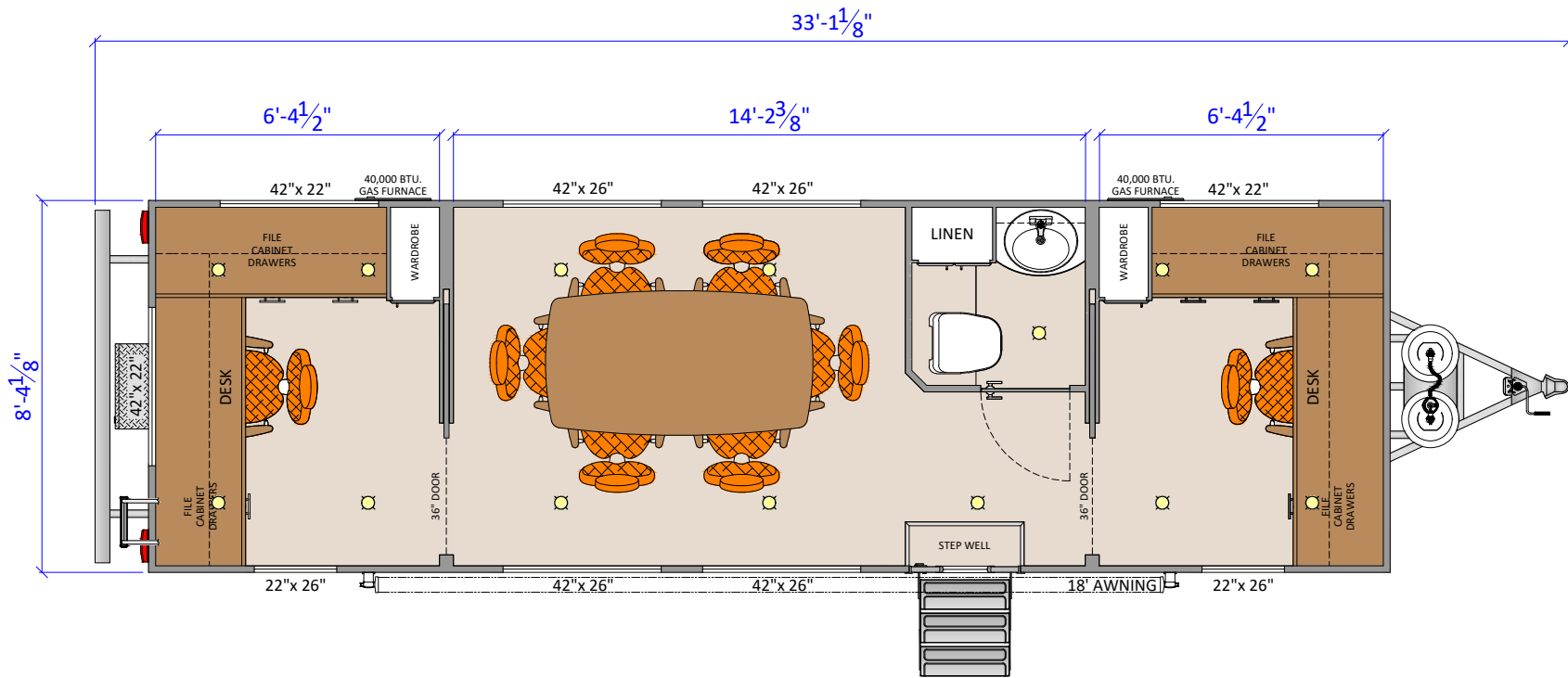
ROUGHNECK (PLAN 105) (290.3 SQ. FT.) TRAVEL TRAILER
