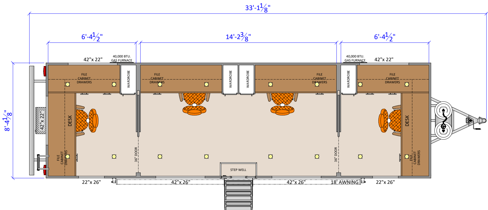
ROUGHNECK (PLAN 104) (290.3 SQ. FT.) TRAVEL TRAILER
