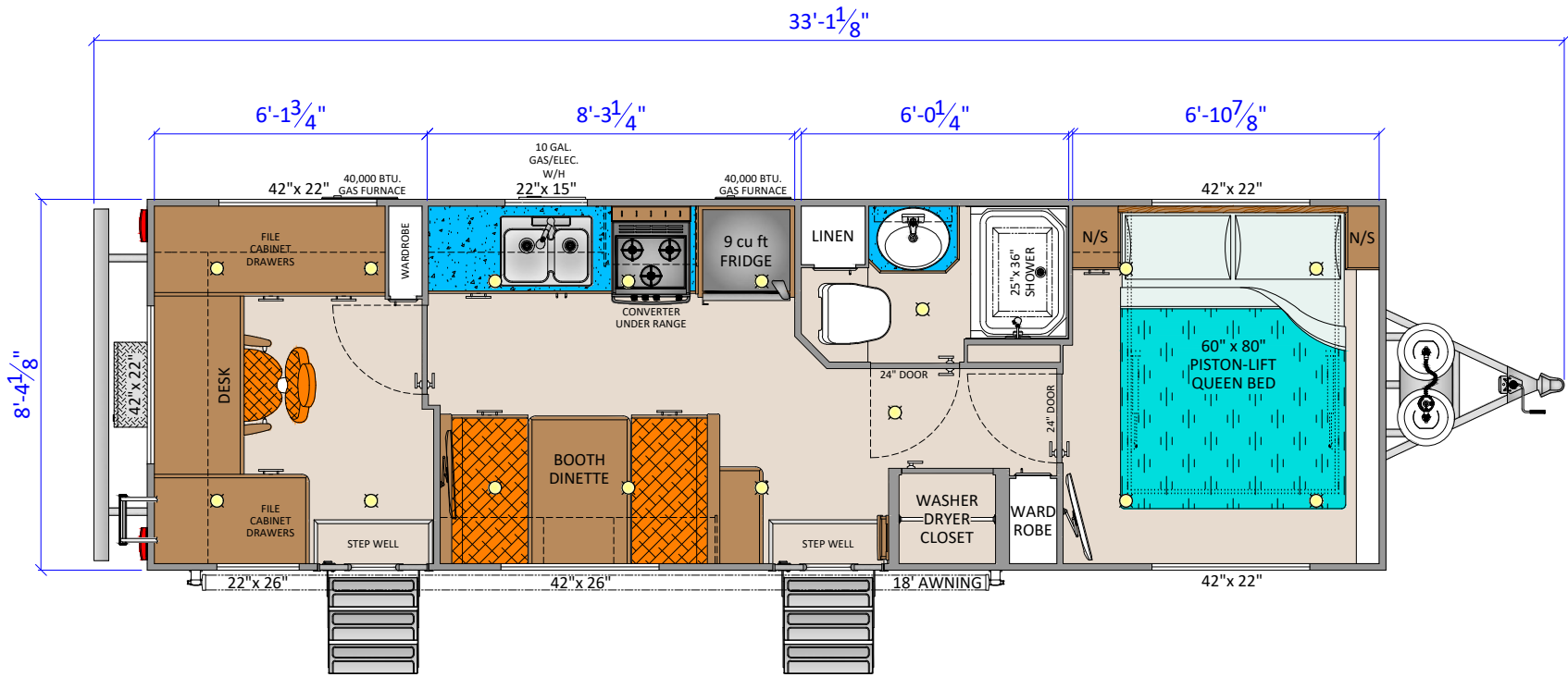
ROUGHNECK (PLAN 103) (290.3 SQ. FT.) TRAVEL TRAILER
