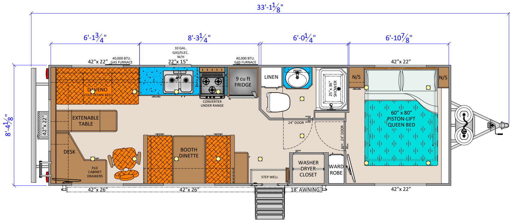
ROUGHNECK (PLAN 102) (290.3 SQ. FT.) TRAVEL TRAILER
