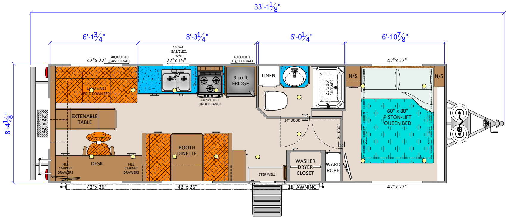
ROUGHNECK (PLAN 101) (290.3 SQ. FT.) TRAVEL TRAILER
