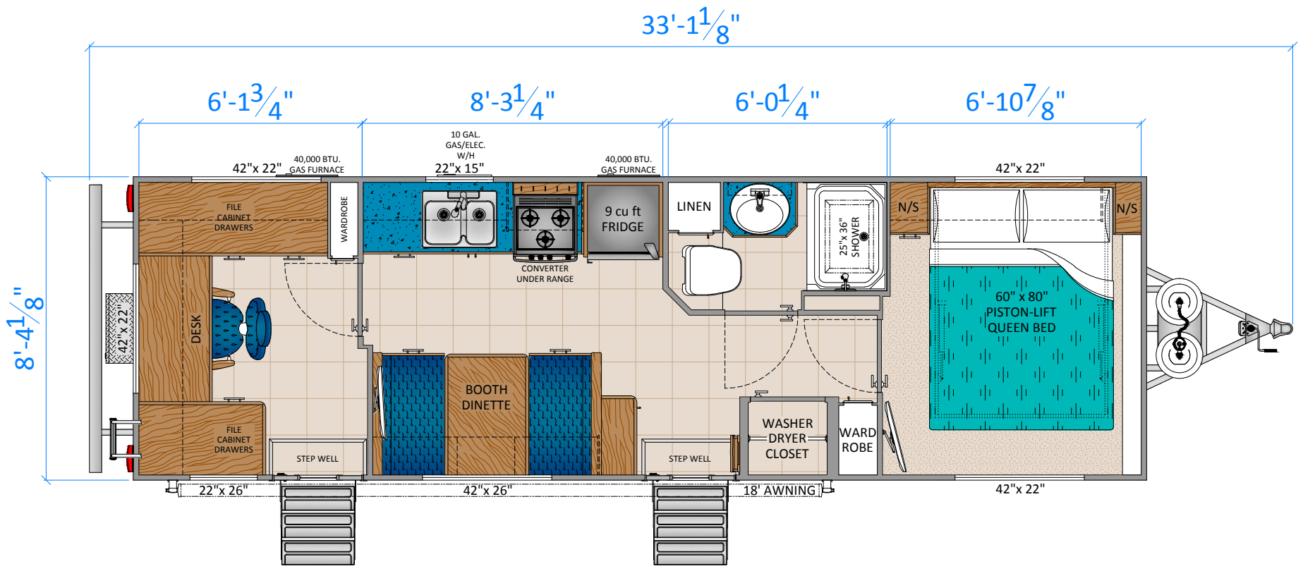
ROUGHNECK (PLAN 103) (290.3 SQ. FT.)
