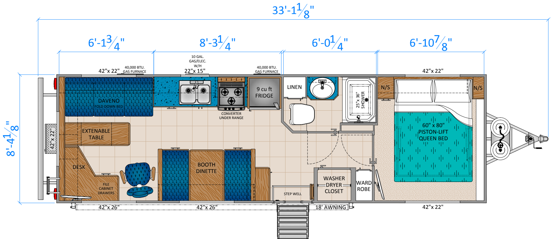
ROUGHNECK (PLAN 102) (290.3 SQ. FT.)
